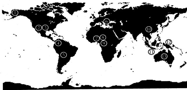
FIG. 1. Geographical map of surveyed human population groups. The figure is a map of the world with the geographic location of all the population groups used in this study denoted by circles with numbers. The populations surveyed were 1, Alaska Natives; 2, United States Caucasians; 3, African-Americans; 4, Arhuaco; 5, Quechua; 6, Greek and Turkish Cypriots; 7, Nigerians; 8, Central African Republic (CAR) Pygmies; 9, Zaire Pygmies; 10, Asians (Vietnamese and Chinese); 11, Indonesians (Nusa Tenggara and Moluccas); 12, coastal and highland Papua New Guineans (PNGs); and 13, Australian Aborigines.
