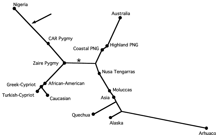
FIG. 2. ML tree of human relationships. This tree was derived directly from the allele frequencies of four polymorphic Alu repeats (TPA 25, APO, ACE, and PV 92) in a total of 664 unrelated individuals (Table 1) using PHYLIP 3.4; the log-likelihood of this tree was 88.936. The distance between population groups is proportional to the branch lengths on the tree. Addition of a hypothetical ancestor that does not contain the Alu repeats results in a branch that connects with the tree at the position denoted by the arrow in the African branch; the asterisk indicates an alternative placement of the root that is not significantly worse than the optimal placement.
